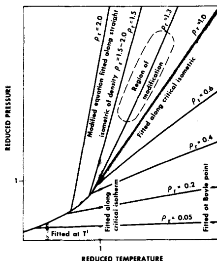
Fig. 1. Typical isometric plot.
